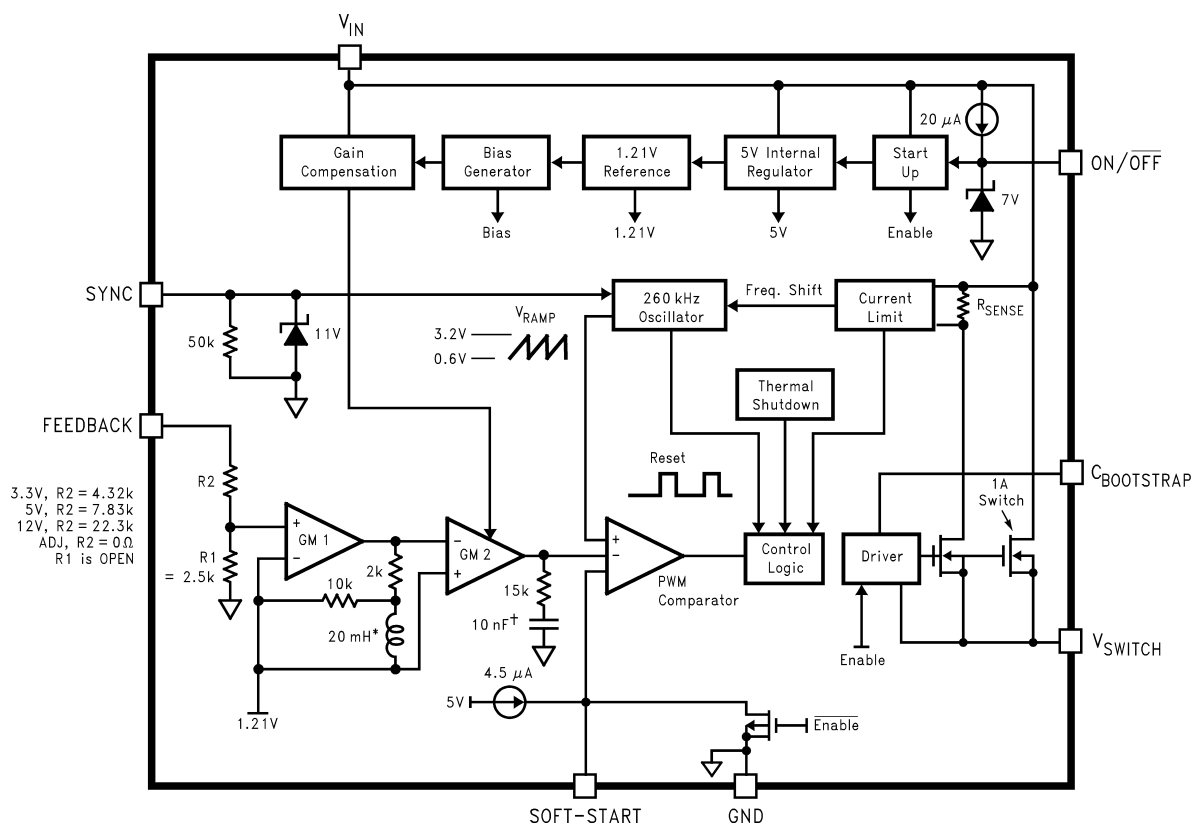
Figure 17. Block Diagram
